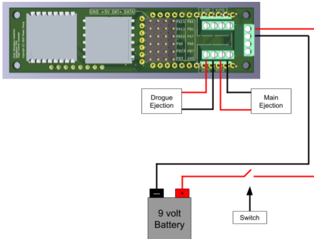
Figure 5: Wiring diagram
